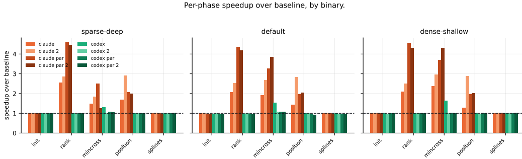
Figure 3: Per-phase speedup. Claude improves ranking, crossing minimization and coordinate assignment on every shape; Codex improves crossing minimization only.
